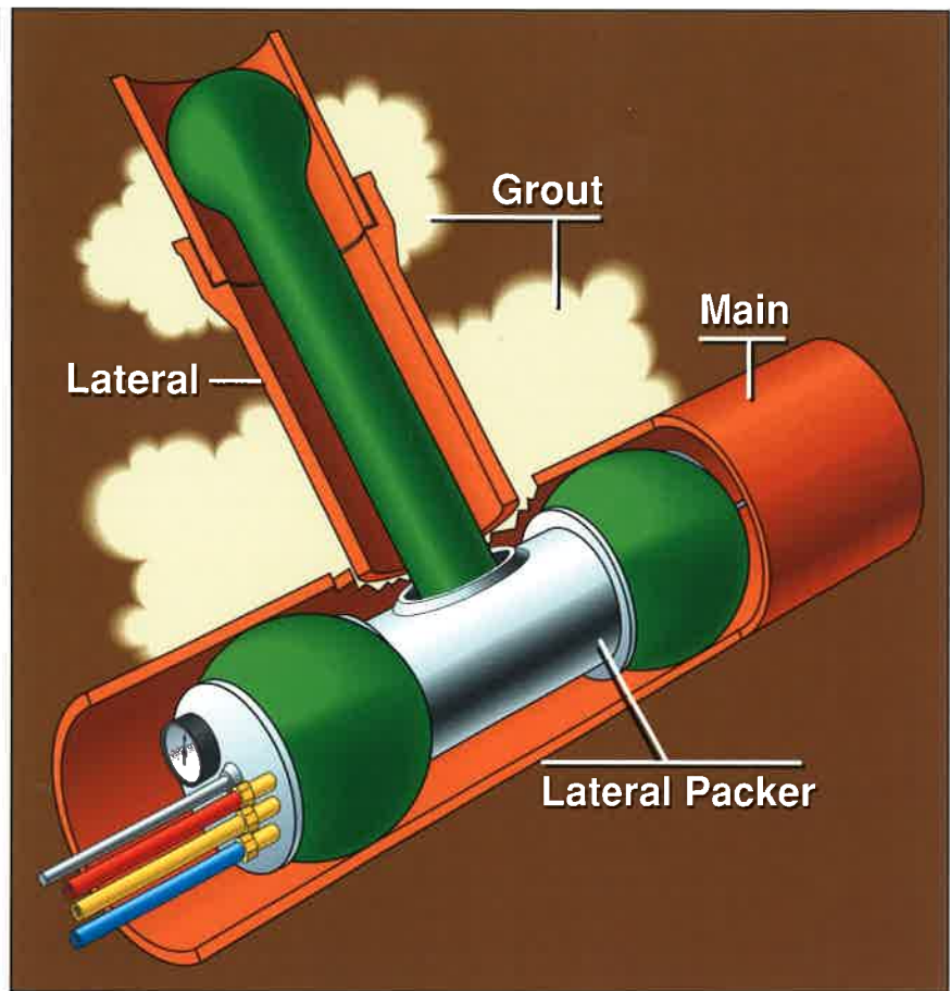
Grout, pumped out through cracks and joints, forms a watertight collar outside the pipeline. Lateral packers are used to seal the connection between laterals and mains, and can seal cracks and joints far into the lateral lines.
